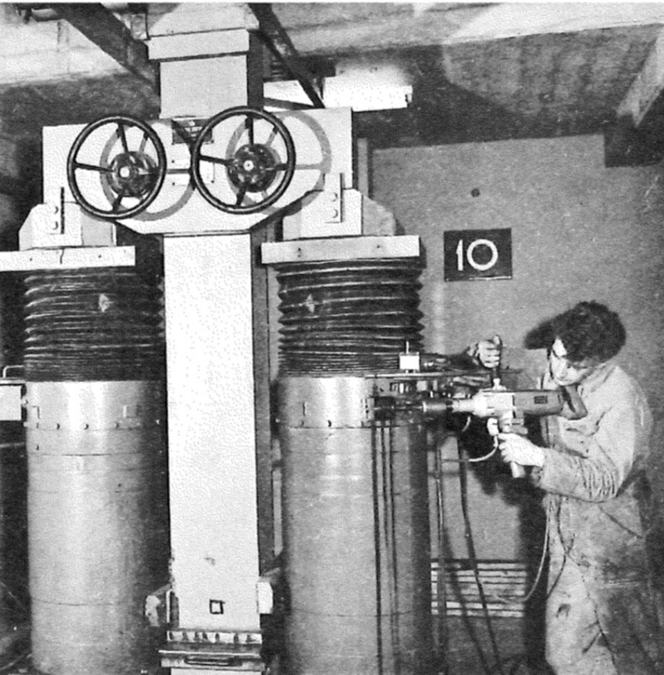
29. Retraction of the jacks while the steel column is supported on steel spacer blocks.
